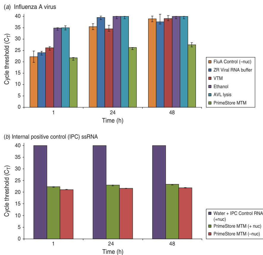
Fig. 1. PrimeStore MTM inactivates nucleases and preserves ( a ) influenza A viral RNA and ( b ) single-stranded internal positive control (IPC) RNA. Real-time RT-PCR analysis was performed using: 10^8 TCID 50 /ml whole influenza A(H3N2) virus preserved in PrimeStore MTM and other media* ( a ), and IPC RNA (preserved in RNA/DNA nucleases (Ambion RNase A, T1, and Turbo DNase) at 37 °C for 48 h. Nucleic acid extraction at 1, 24 and 48 h was performed and PCR amplified using PrimeMix Universal Influenza A and PrimeMix IPC assays (Longhorn Vaccines & Diagnostics). Mean and standard error bars for duplicate extractions are shown. A C_T reading of 40 ( C_T=40 ) is no amplification. [* Viral transport media (VTM) is BD Universal Viral Transport Medium for Viruses, Chlamydiae, Mycoplasmas and Ureaplasmas (BD, USA); AVL Lysis Buffer is Buffer AVL viral lysis buffer (Qiagen, cat. no. 1014777; USA). ZR Viral RNA Buffer is from Zymo Research (cat. no. R1034-1-50).]
